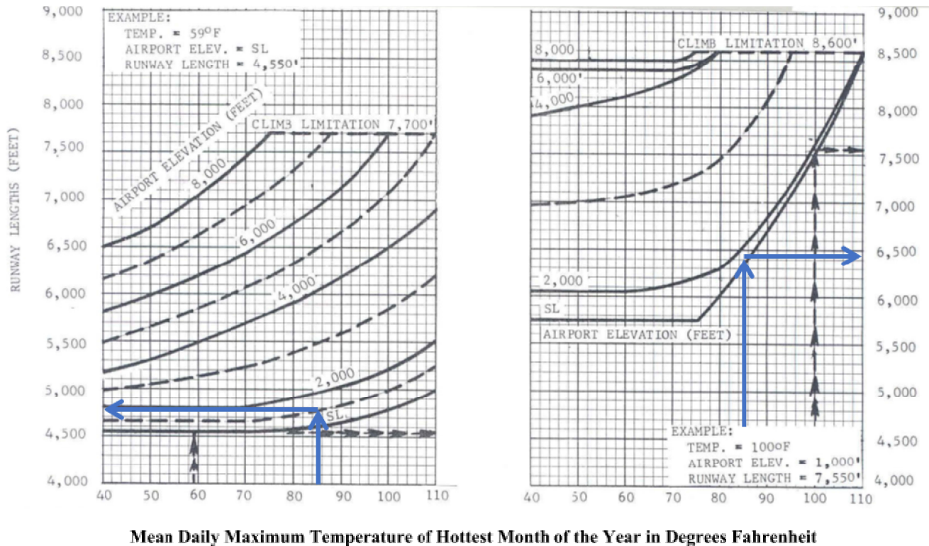
Figure 3.1: Required Runway Length to Accommodate 75% of Fleet
