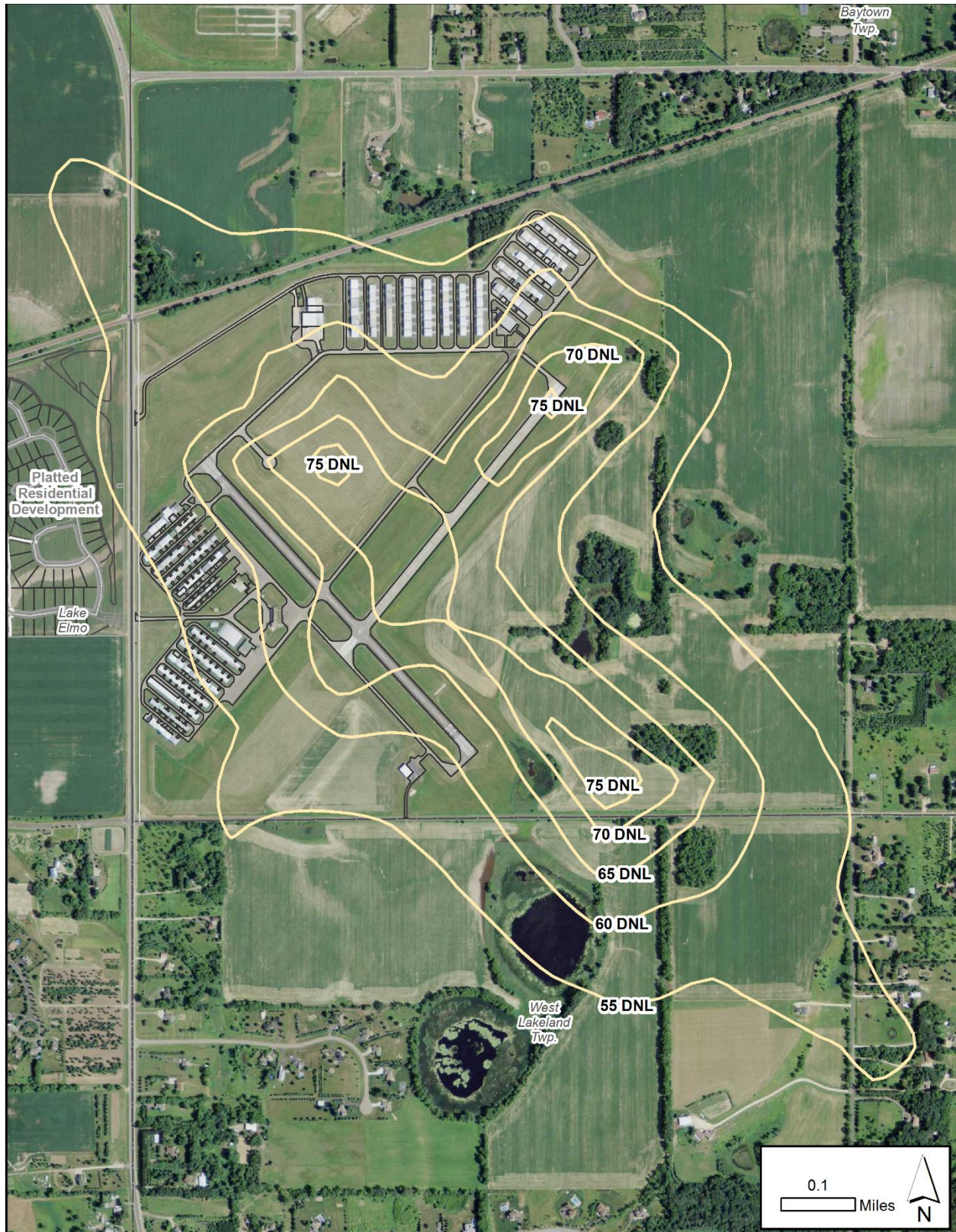
Figure 6-4: 2035 Final Preferred Alternative Noise Contour
