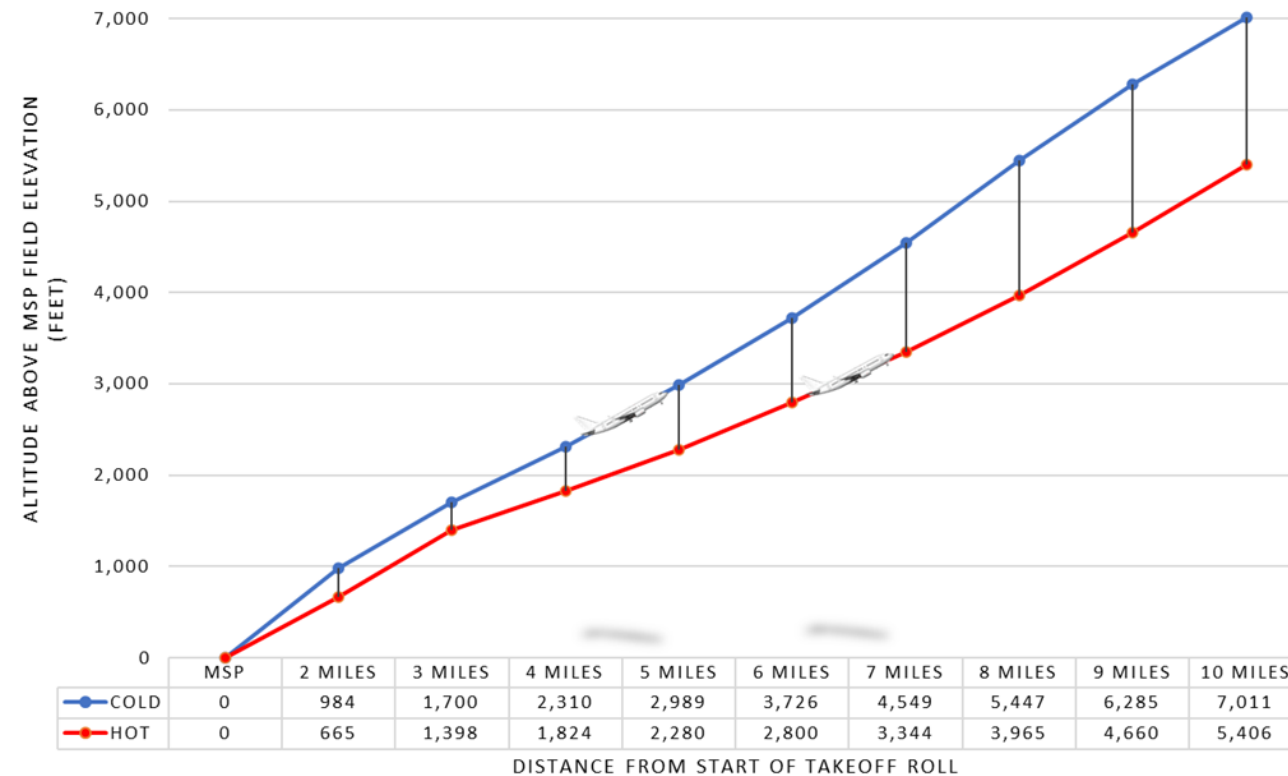
MSP AVERAGE DEPARTURE CLIMB ALTITUDES
