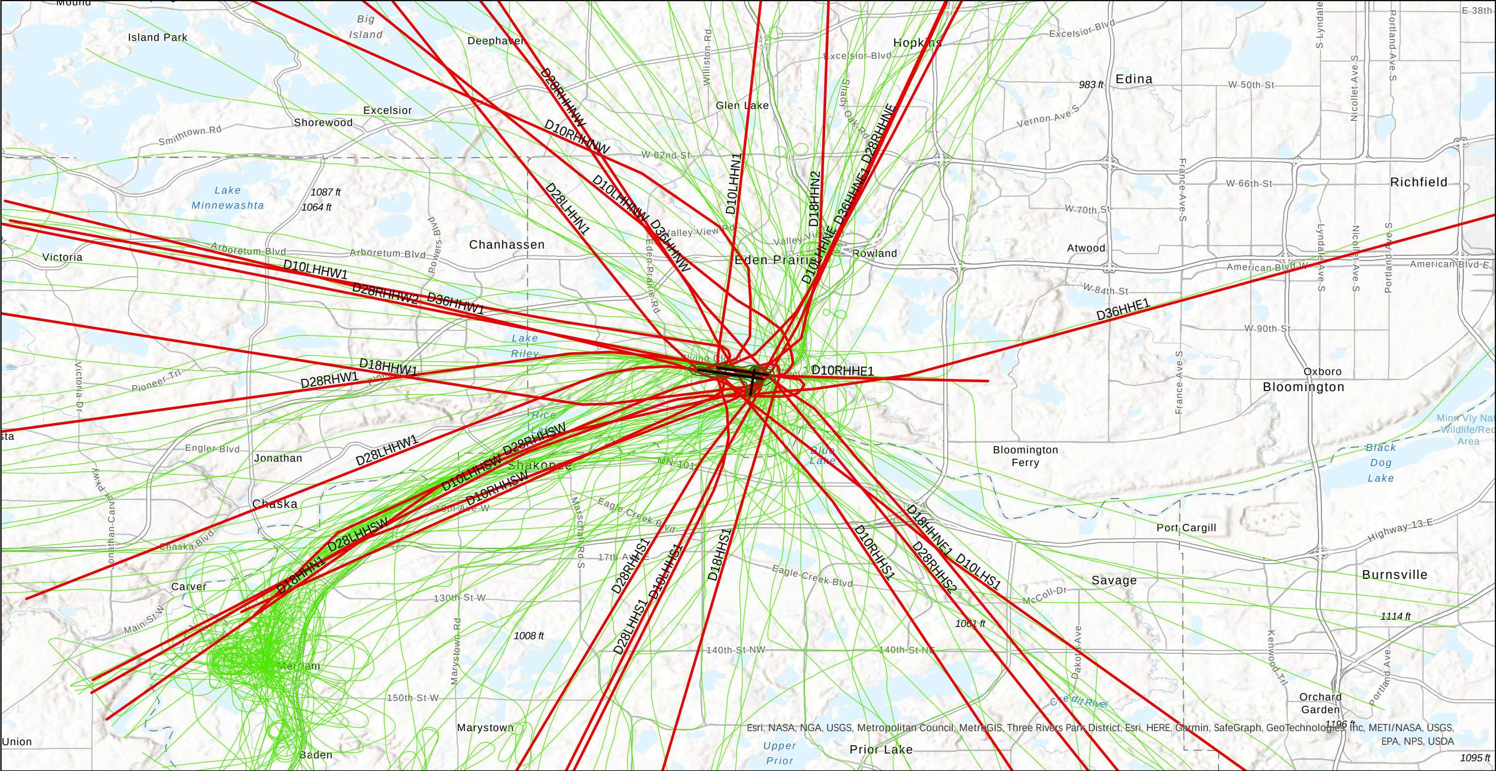
Figure 38 DEPARTURES - HELICOPTER
