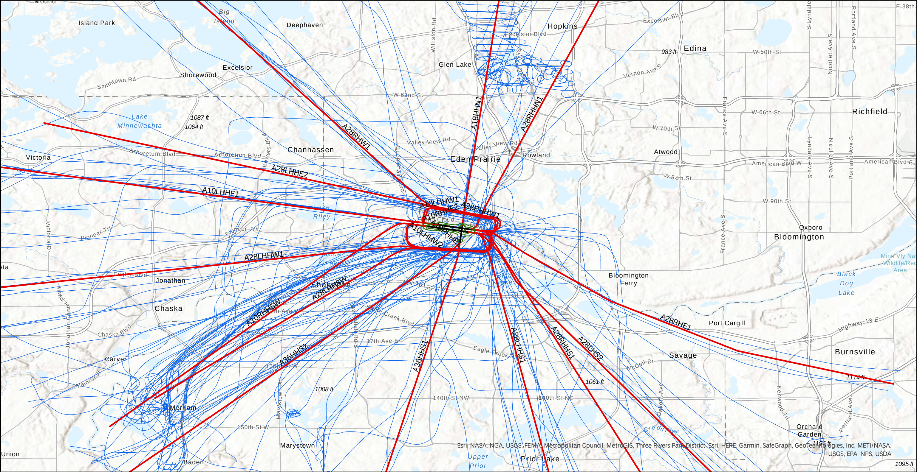
Figure 37 ARRIVALS - HELICOPTER
